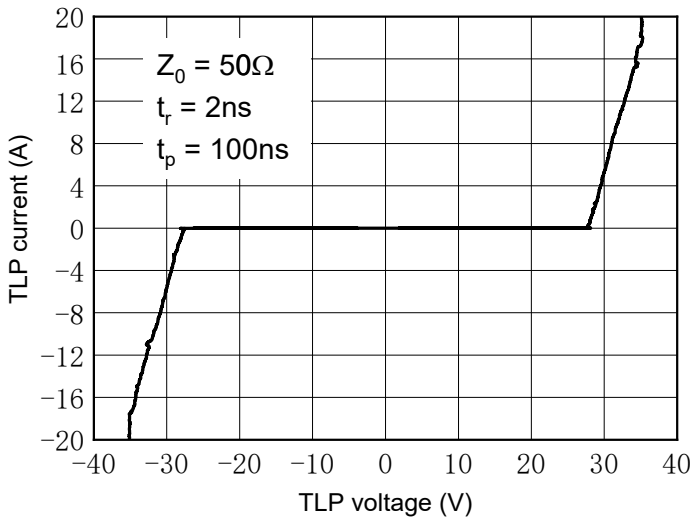
Fig.7 TLP Measurement
